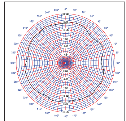
F11 - TYPICAL H-PLANE
