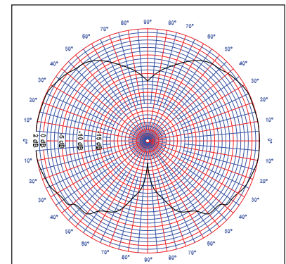
F11 - TYPICAL E-PLANE
