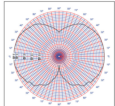
F11 - TYPICAL H-PLANE
