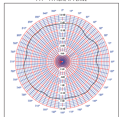
F11 - TYPICAL H-PLANE
