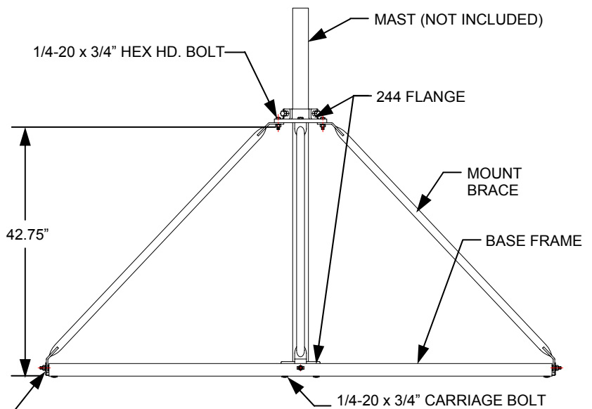
Figure 2 (Front View)
