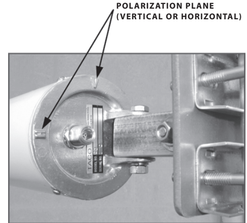
MOUNT DETAIL
